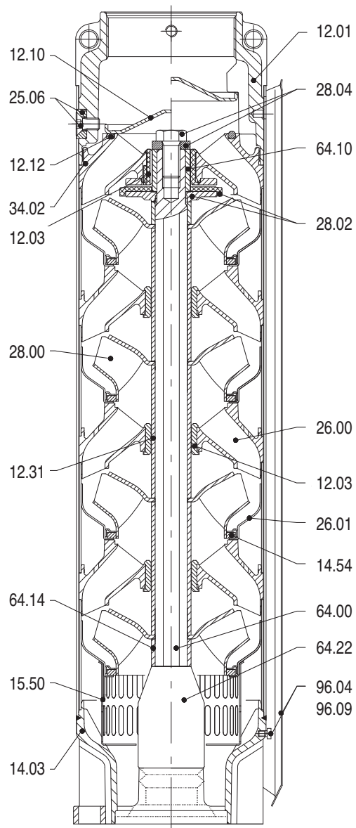
6SDX 45 6SDX 60 Mixed flow pump
