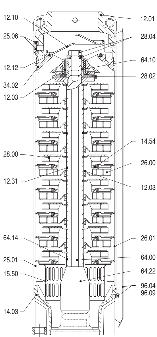
6SDX 13 6SDX 18 6SDX 27 Radial flow pump
